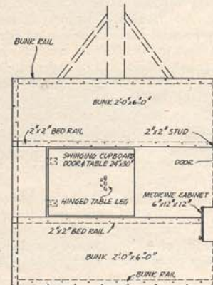
2 BUILT-IN ARRANGEMENT
